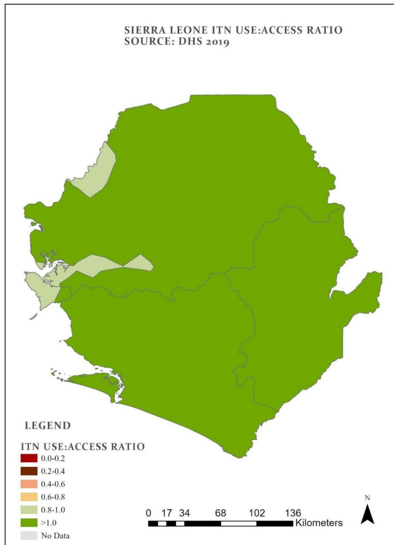
Figure 5. ITN Use:Access Ratio Map
